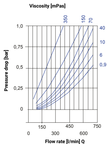
Typical pressure drop V0115
